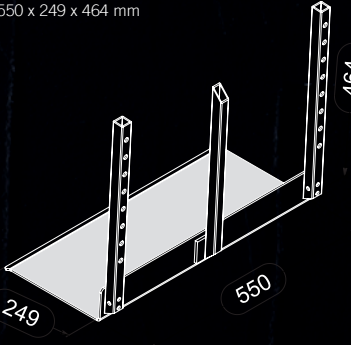
25 cm - Holme normal 550 x 249 x 464 mm
