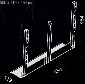
Standard 12 cm - Holme normal 550 x 119 x 464 mm
